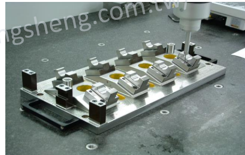
CYLINDER HEAD MASTER
