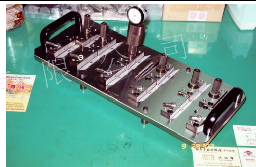
CYLINDER HEAD 油穴孔位檢具
