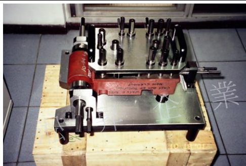
HOUSING 孔位檢具
